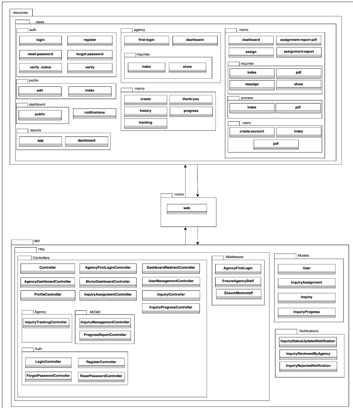
Figure 3.4 Model View Controller (MVC) Package Relationship for My Sebenarnya Systems
