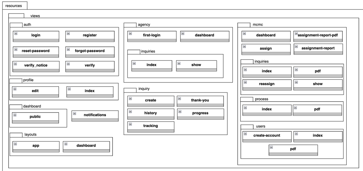
Figure 3.1 Application Layer for MySebenarnya Systems
