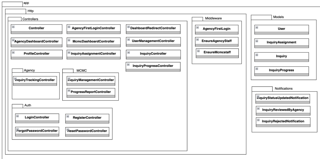
Figure 3.2 Business Services Layer for MySebenarnya Systems
